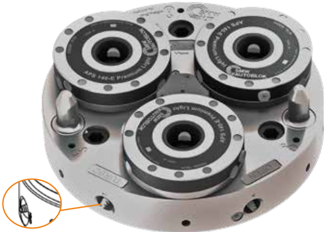
N. 2 PNEUMATIC CONNECTIONS FOR MANUAL OPENING AND TURBO COMMAND
