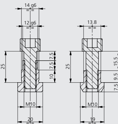
T-SLOT 14 46204104
