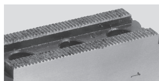
Dirty/damaged serration
