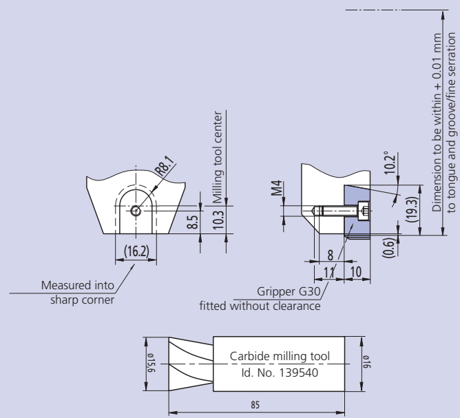
Mounting dimension
