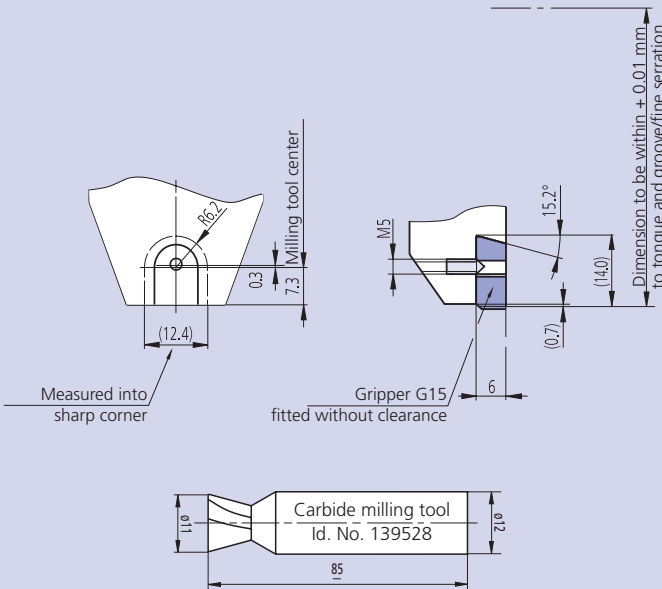
Mounting dimension
