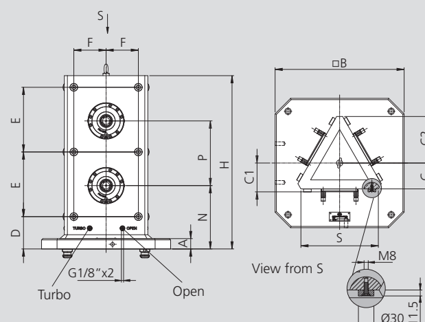
Tombstone with 6 APS modules
