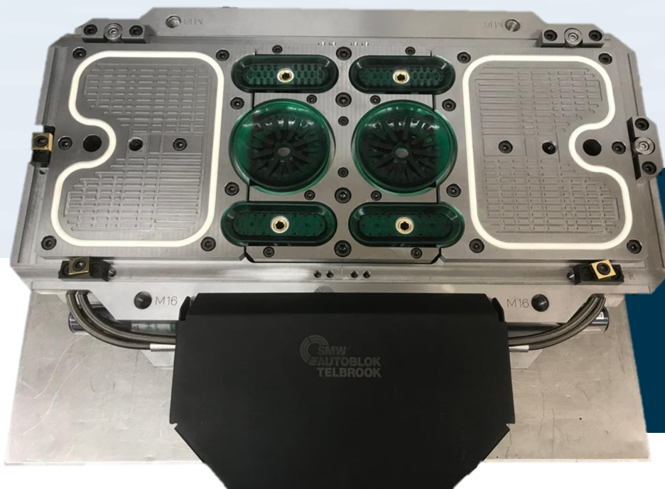
Vacuum Fixtures
